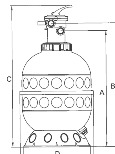
Quote filtri HI Top
