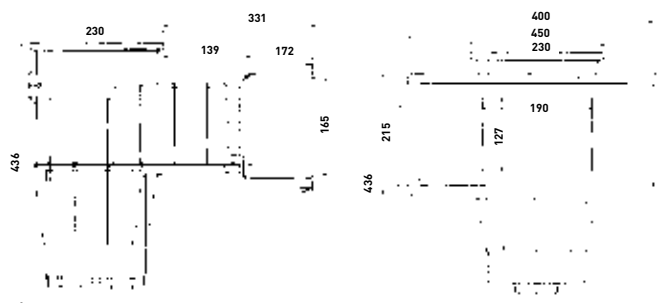
Skimmer grande meurtrière - Wide face opening skimmer
